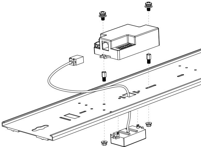
FINAL ASSEMBLY
