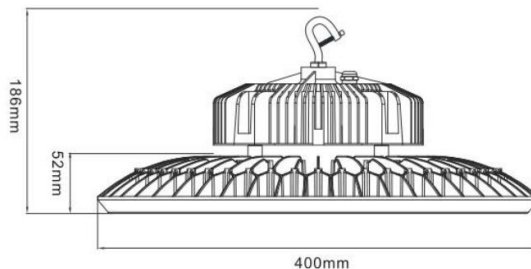
200-240W Dimension
