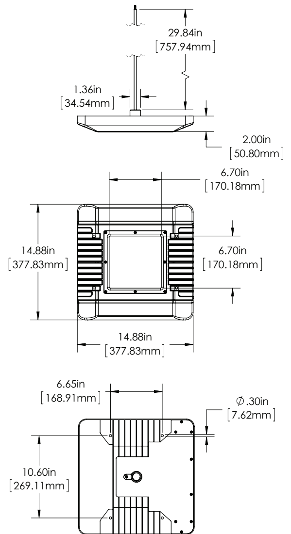
INSTALLATION DRILL LAYOUT
