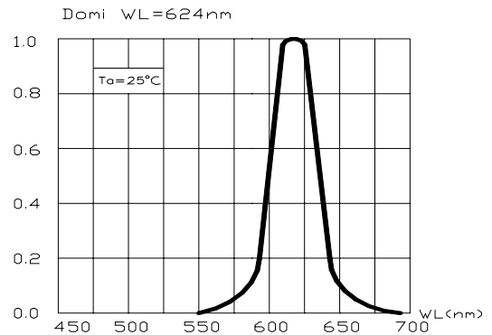
Fig.4 Relative Luminous Flux vs. Wavelength
